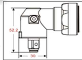
OP-301LB90 3/8" Rear exhaust 後排氣
